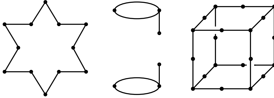
FIGURE 4. The discretizations of the configuration spaces in Examples 1-3 (left to right).
